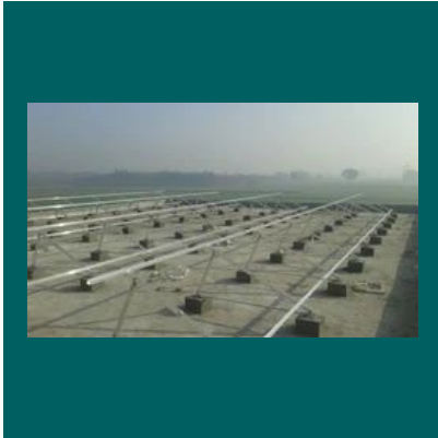
Aluminum Solar Module Mounting Structure
